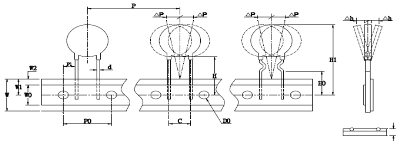
Fig. 2 For KRL2400025 - KRL2400055, KRL2400075, KRL2400135
