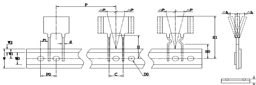
Fig. 4 For KRL2400200
