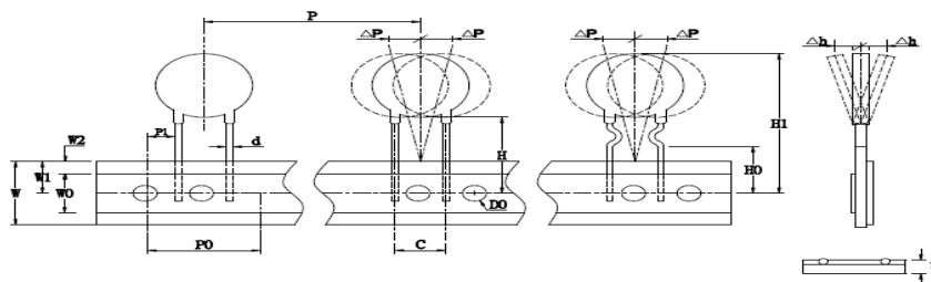
Fig.3 For KRL1200300
