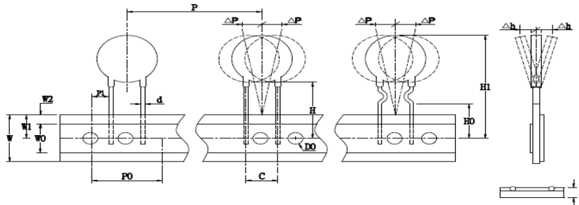
Fig. 4 For KRL2400200
