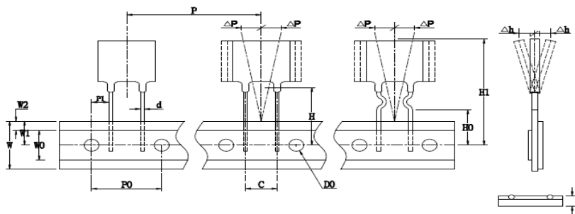
Fig.3 For KRL1200300
